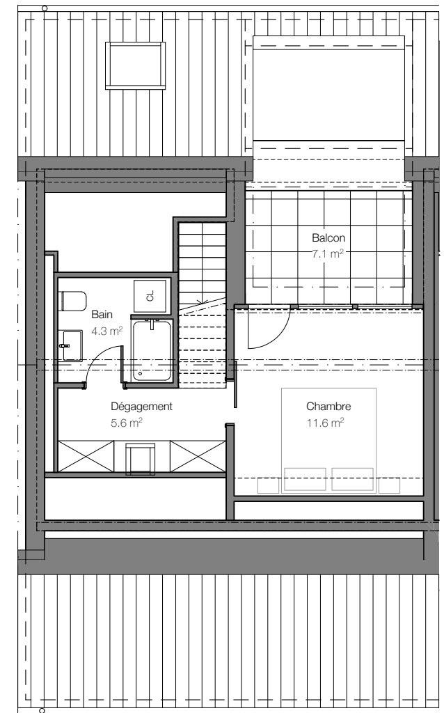
Combles
