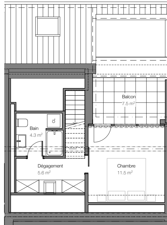
Combles
